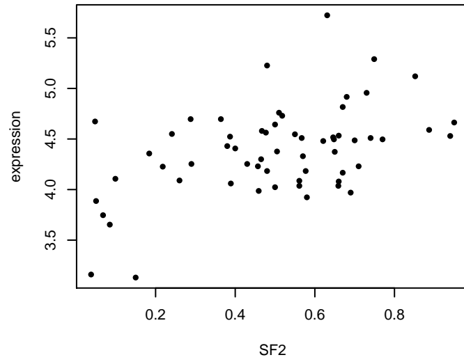
SQSTM1 : Corr = 0.483
