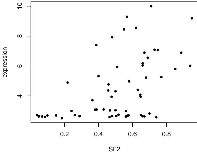
HTRA1 : Corr = 0.517
