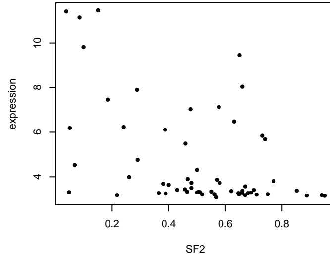
ARHGDI3 : Corr = -0.487
