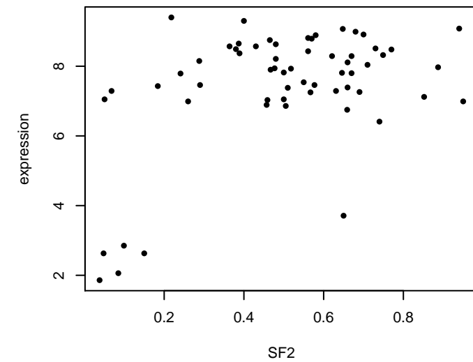
PTMS : Corr = 0.476
