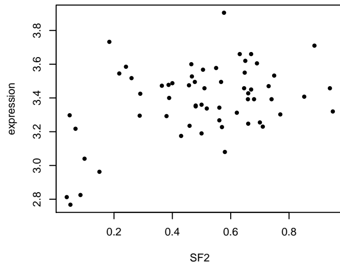
TWF1 : Corr = 0.422
