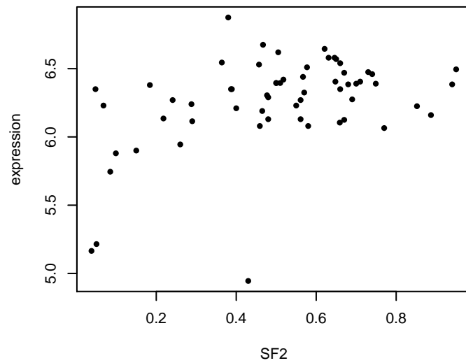
PKM2 : Corr = 0.446
