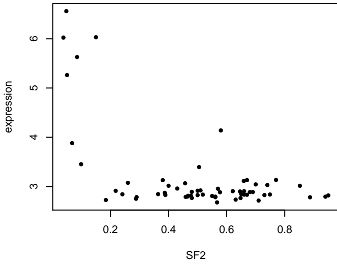
MYB : Corr = -0.593
