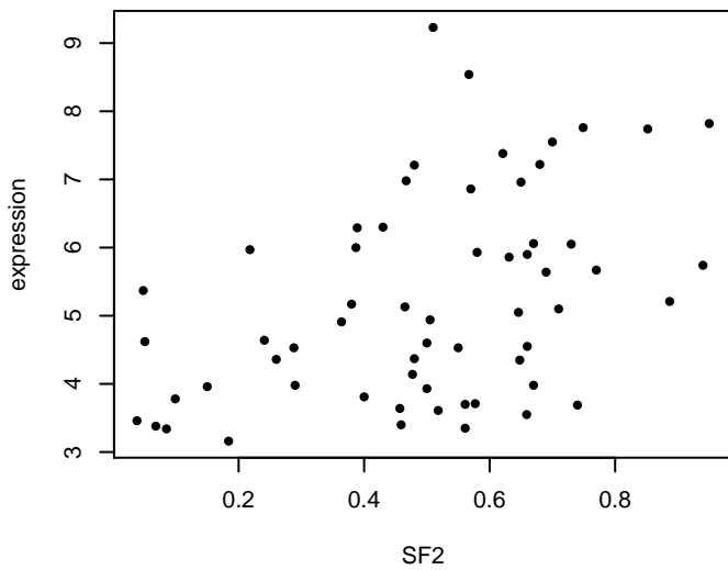
PIR : Corr = 0.432
