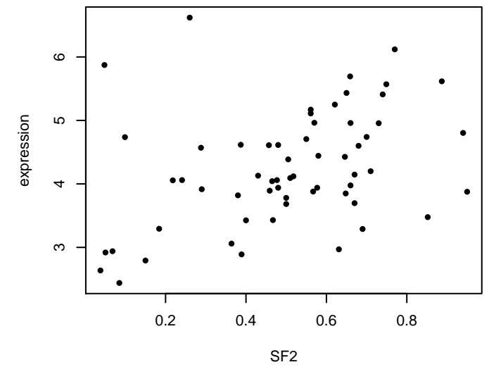
EMP2 : Corr = 0.372
