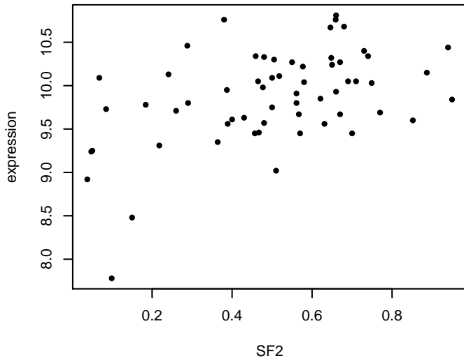
CAPNS1 : Corr = 0.482
