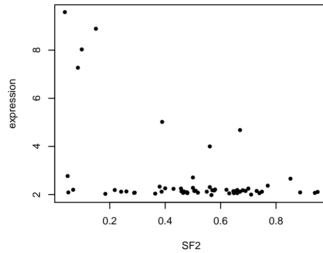
CXCR4 : Corr = -0.459
