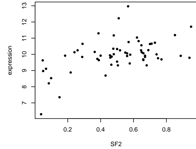
CD63 : Corr = 0.509
