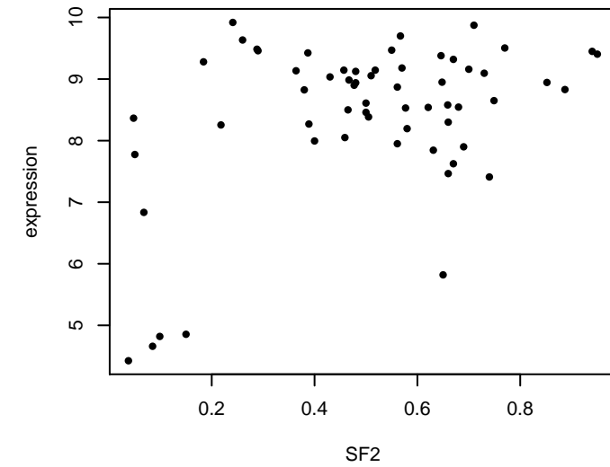
RAB13 : Corr = 0.423
