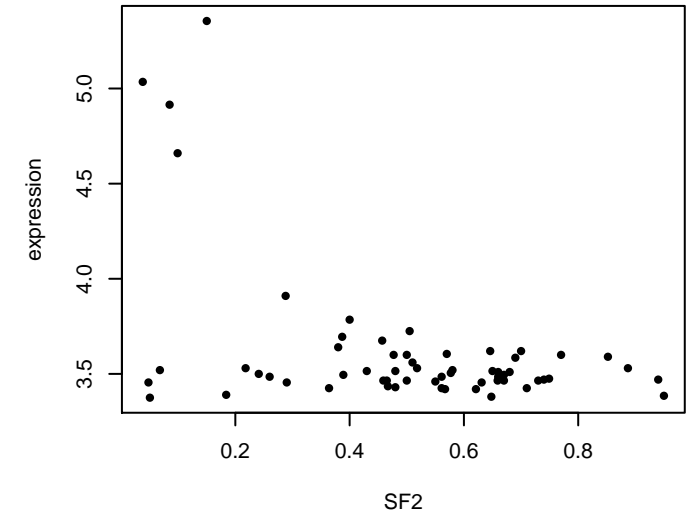
LRMP : Corr = -0.473
