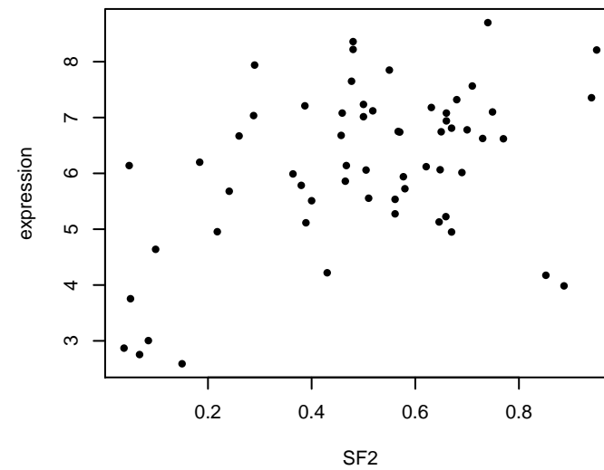
ITGB5 : Corr = 0.462
