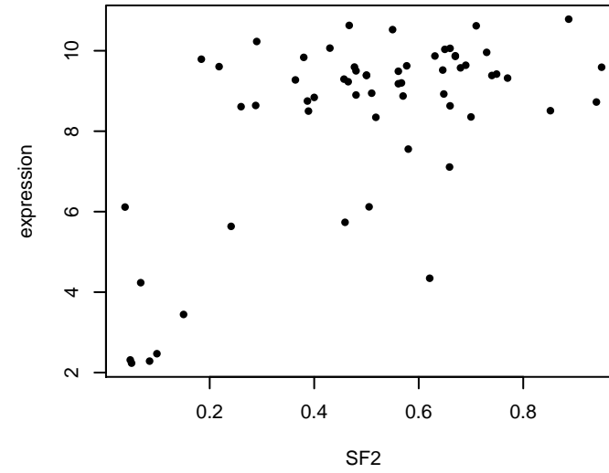
PFN2 : Corr = 0.614
