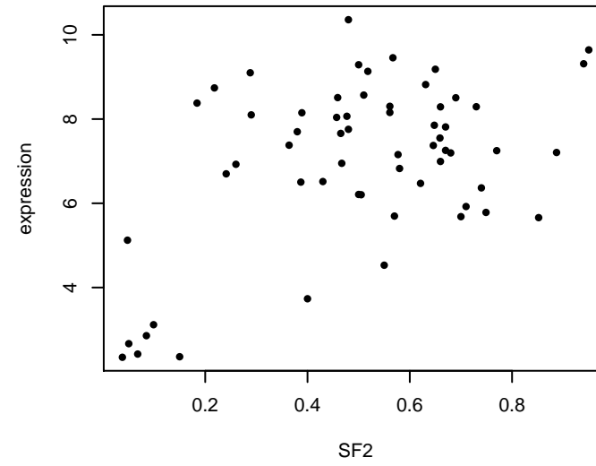
CCND1 : Corr = 0.499
