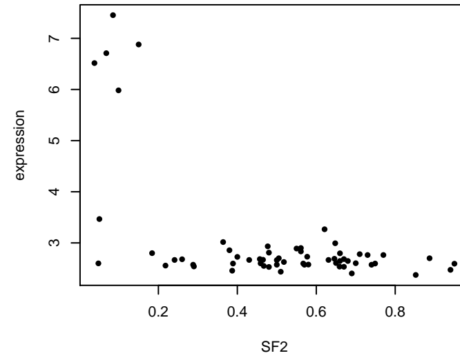
WAS : Corr = -0.572
