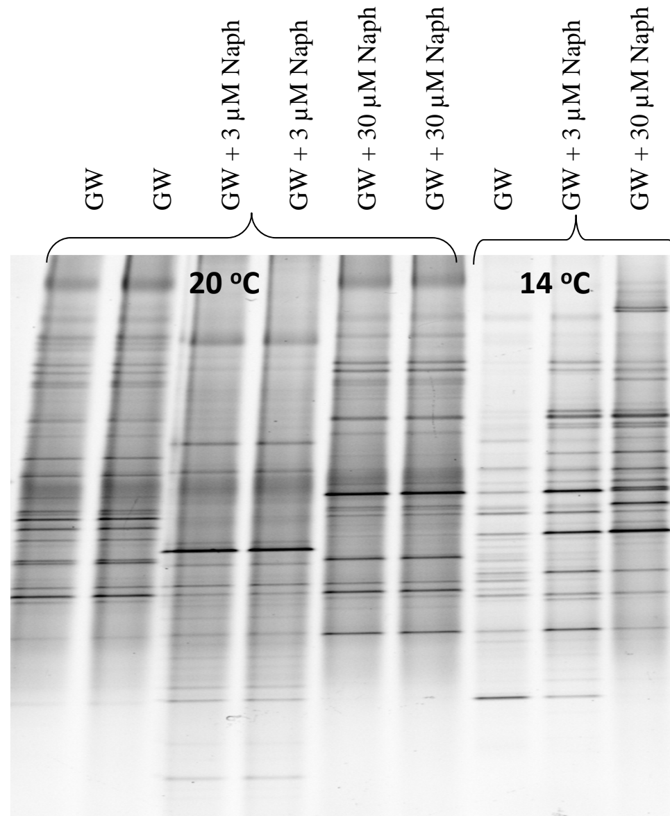
Figure S2. The effect of temperature and naphthalene concentration on the structure of the microbial community determined by 16S rRNA DGGE analysis.
