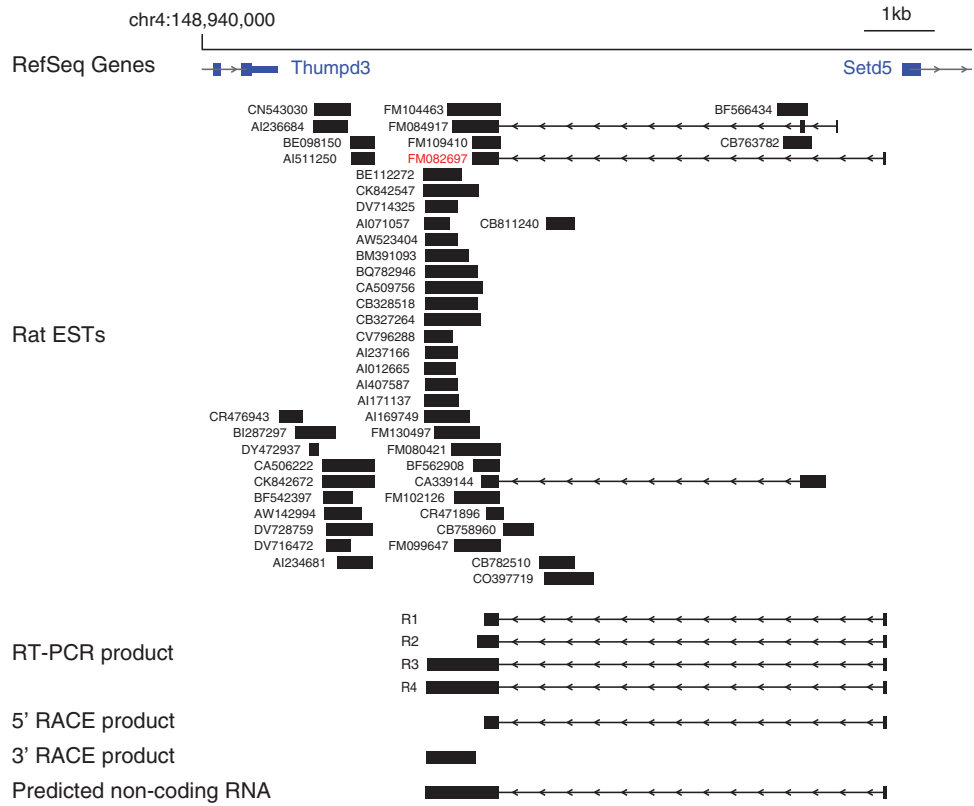
SUPPLEMENTARY FIG. S2. Rosa26 Loci and ESTs from Database in rat genomes. EST, expressed sequence tag; RACE, rapid amplification of cDNA ends; RT-PCR, reverse transcription-polymerase chain reaction.
