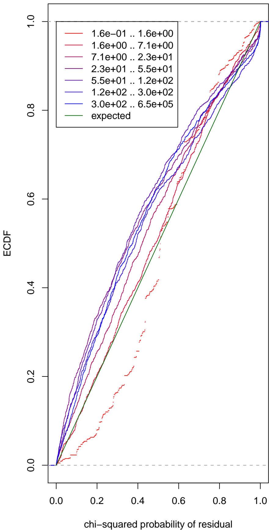
Residuals ECDF plot for condition 'H'
