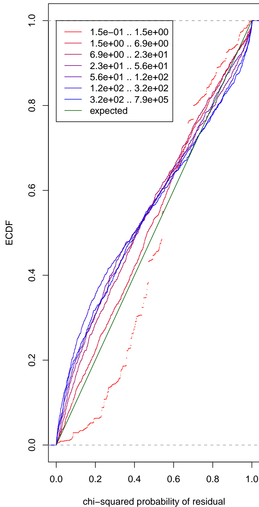
Residuals ECDF plot for condition 'L'
