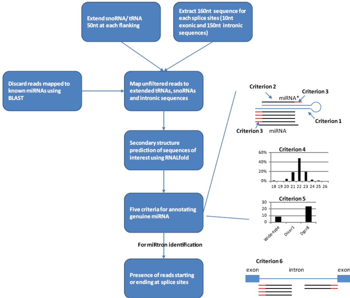
Supplemental Figure S1. Flowchart describing the major steps for novel miRNAs identification.
