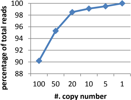
Supplemental Figure S8. The relationship between the copy number and the percentage of all genomic-aligned reads included
