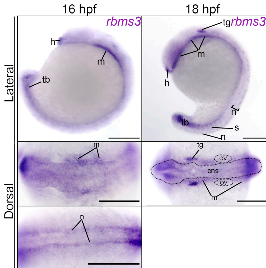
Figure S1. Expression for rbms3 at 16 and 18 hpf expands to the nervous system and cranial mesenchyme. Lines and brackets highlight expression. cns, central nervous system; h, hatching gland; m, cranial mesenchyme; n, neurons; ov, otic vesicle; s, somites; tb, tail bud; tg, trigeminal ganglion. Bars, 200 \mu M.
