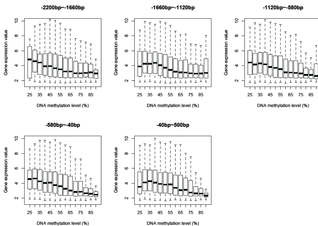
Figure S1 Relationship between DNA methylation in regions of different distances to transcriptional start sites and gene expression levels in the human cerebral cortex.
