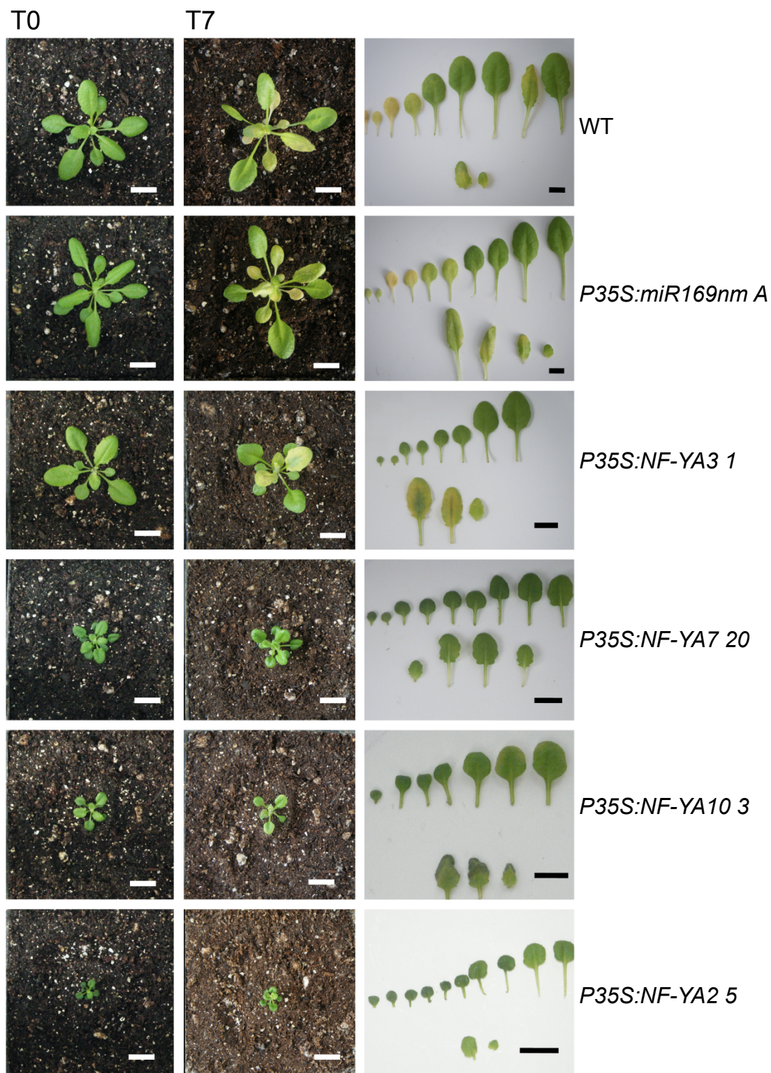
Figure S12. NF-YA overexpression delays dark-induced senescence.
