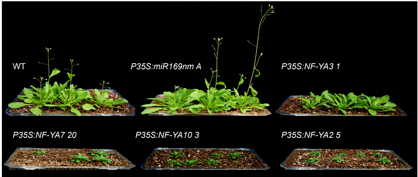
Figure S16. NF-YA overexpression delays flowering time.
