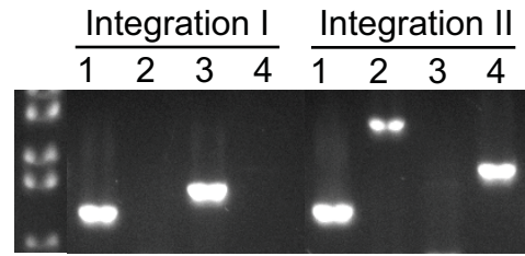
PCR analyses of integration sites
