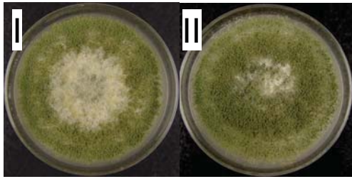
Two types of colony morphology on PDA
