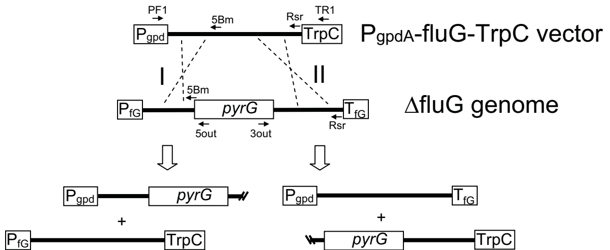
Schematic representation of the two types of integration
