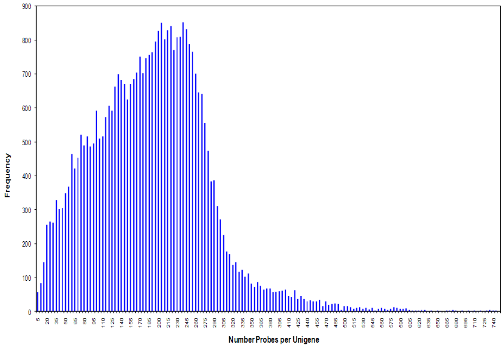
Figure S2 A histogram showing the number of probes per unigene.
