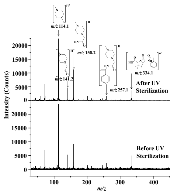
Figure S2: MALDI-MS/MS of the m/z 490.2 protonated parent from MPA-ampicillin adsorbed on chitosan-alginate polyelectrolyte multilayers before and after UV sterilization.
