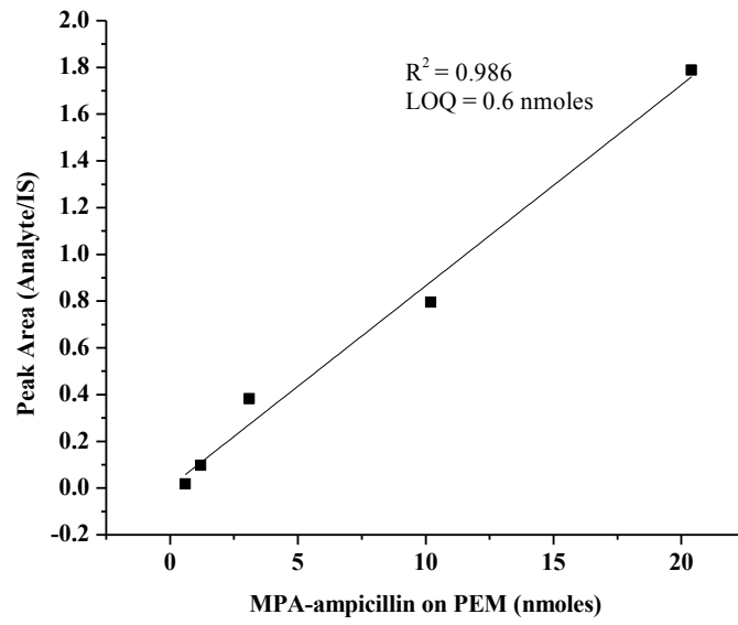
Figure S3: Linear regression plot for MPA-ampicillin adsorbed on chitosan-alginate polyelectrolyte multilayers with sulfadiazine as internal standard.
