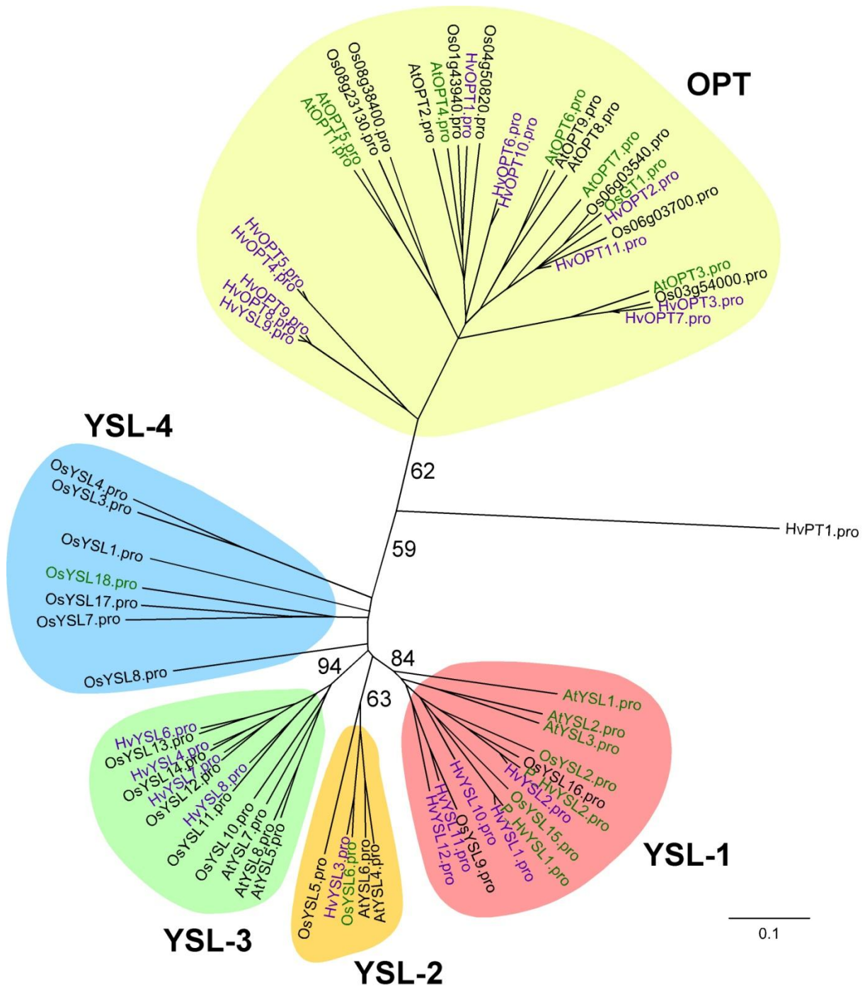
Additional Figure 5 Detailed phylogenetic tree of plant OPTs. Clustering of 17 Arabidopsis, 26 rice and 24 barley sequences (accounting for 22 unique sequences). To support the tree, barley full-length sequences from H35 and publications were included. Barley sequences are written in violet, functionally characterised transporters in dark green (see Additional Table 2)
