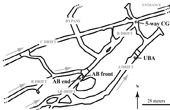
FIG. S1. Map of mine showing sampling locations
