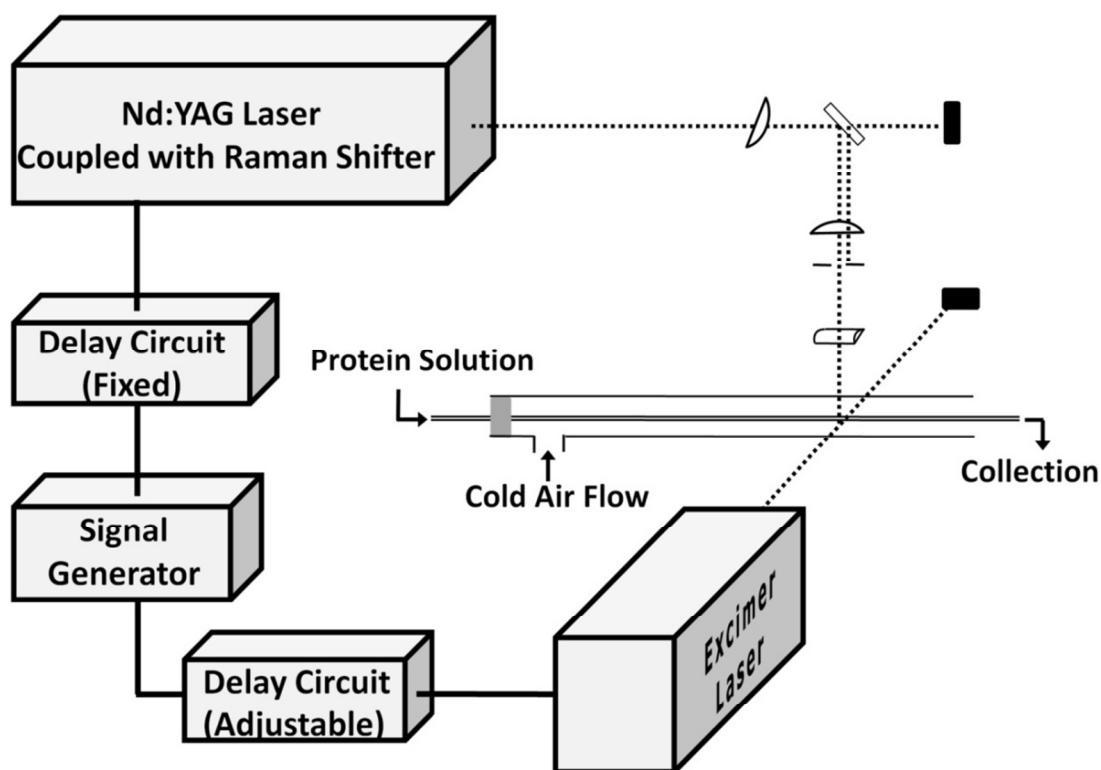
Figure S1: Schematic of the “pump-probe” system (taken from reference 29)
