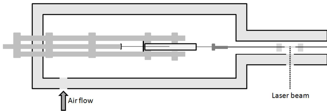
Figure S2: Schematic of the 2 nd chamber of the temperature-control system (taken from the Ph.D.
