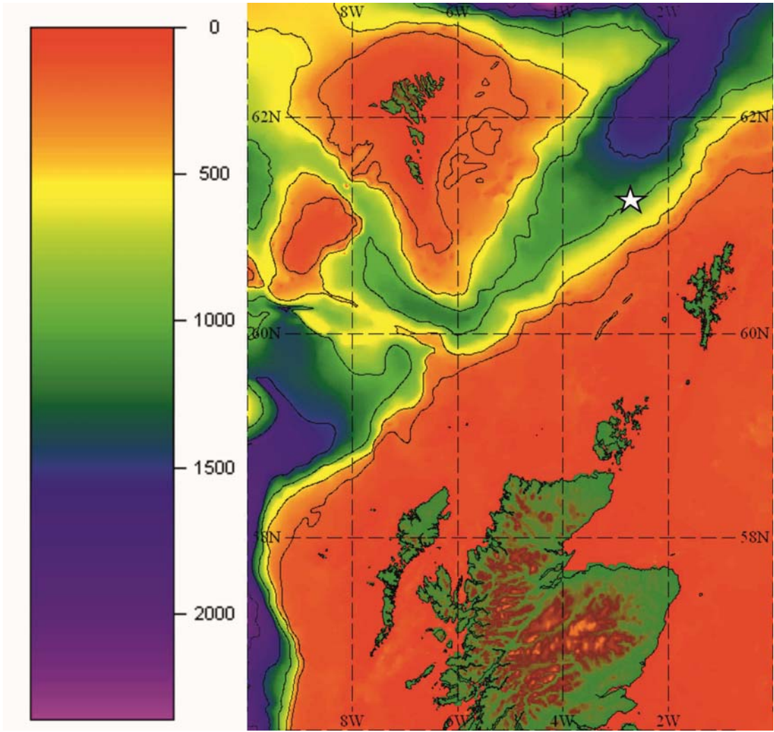
Figure S1. Map illustrating the location of the sampling site (white star) in the Faroe Shetland Channel, Northeast Atlantic. Inset legend denotes water depth in metres.
