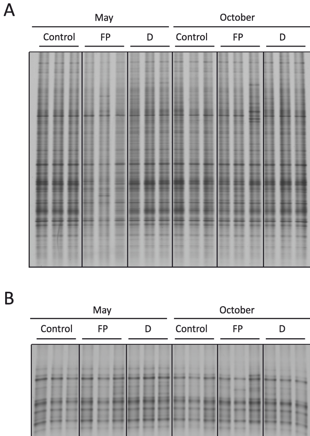
Figure S4. DGGE analysis of bacterial (A) and archaeal (B) community structures in the upper 1 cm of sediment from the control, faecal pellet (FP) and diatom (D) treatments in May and October. Each vertical track represents a replicate sediment core ( n = 3 in all cases).
