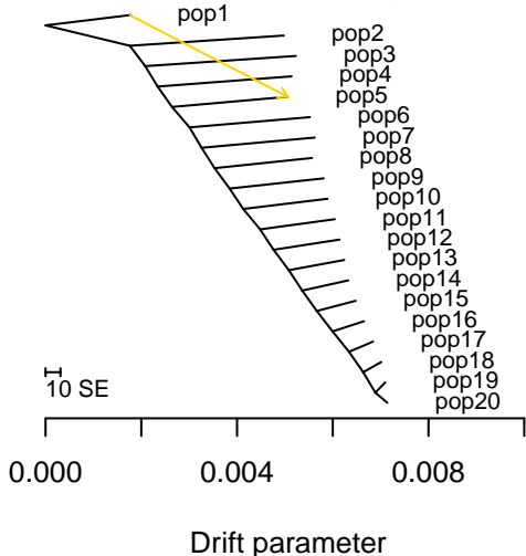
A. correct graph topology
