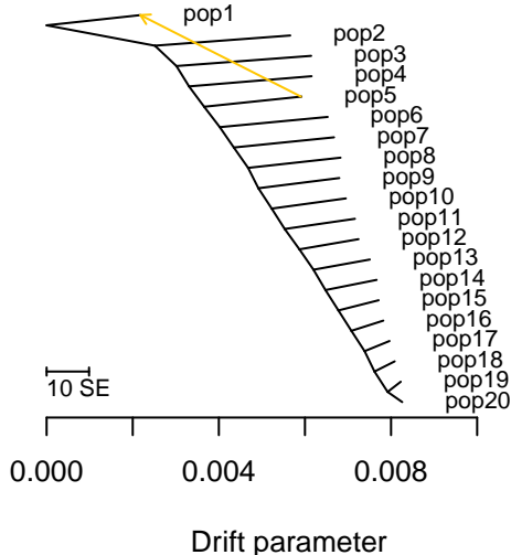
B. common error (w = 10%)
