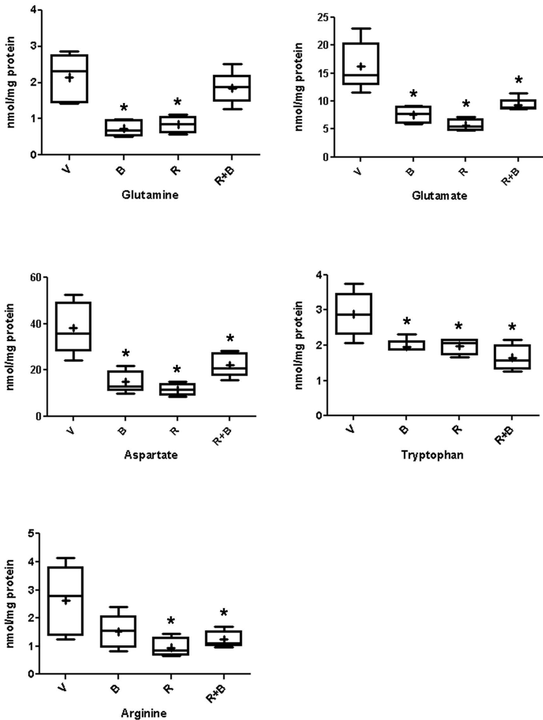
Figure S5. LC-MS/MS validation for selected metabolites. Whiskers represent minimum and maximum values. The bar represents the median value, and the plus sign the mean value for n = 4 to 5 lung samples from individual mice after 2 weeks of drug treatment. The asterisk indicates p < 0.05 for individual treatments compared to the average vehicle score.
