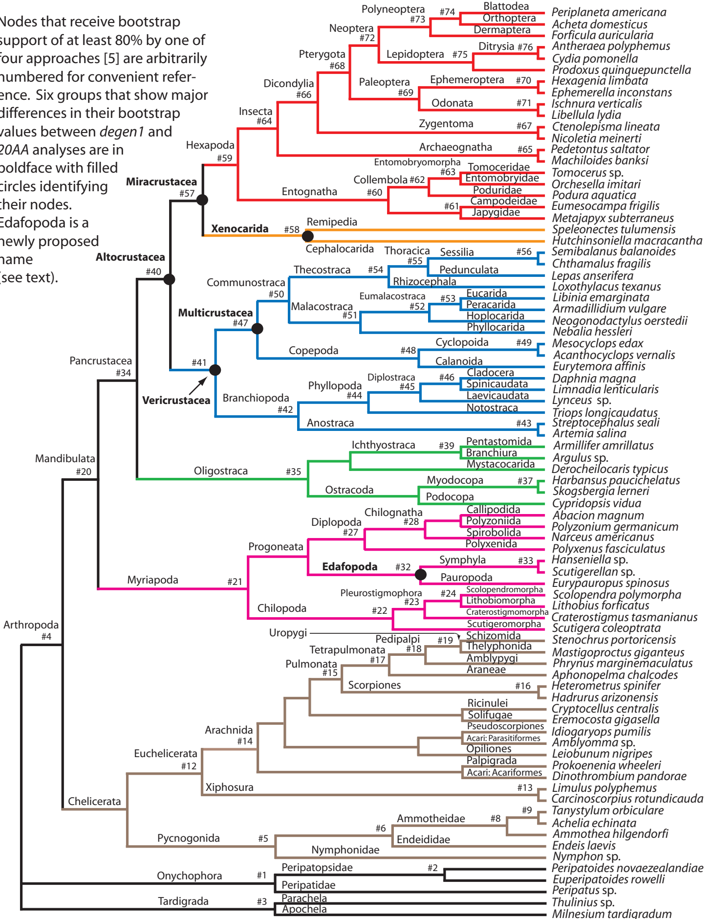
Figure S1. Arthropod relationships and classification scheme based on degen1 analysis of 75 ingroup plus five outgroup species [5].
