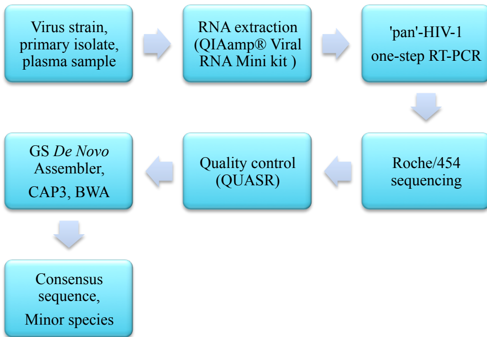
FIG S1 Flowchart of the universal method for generation of HIV-1 genome sequences. QUASR is freely available at http://sourceforge.net/projects/quasr/ .
