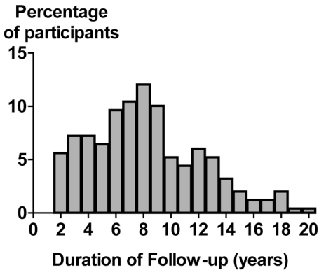
Figure 1. Distribution of follow-up duration for study participants. Frequency histogram of ophthalmic follow-up duration for the 249 participants in the current study. The mean follow-up time was 8.2 \pm 4.0 years, with a median follow-up time of 7.7 years (range 2.1 to 19.8 years).
