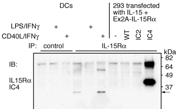
Supp. Figure 10. Detection of IL-15R \alpha -IC4 in human dendritic cells. Antisera directed against IC4 were developed in rabbits and used to re-hybridize the membrane as shown in Figure 6. IL-15R \alpha -IC4 appeared to be expressed at the expected size (arrow) in immature as well as in dendritic cells matured with IFN- \gamma plus CD40 ligand.
