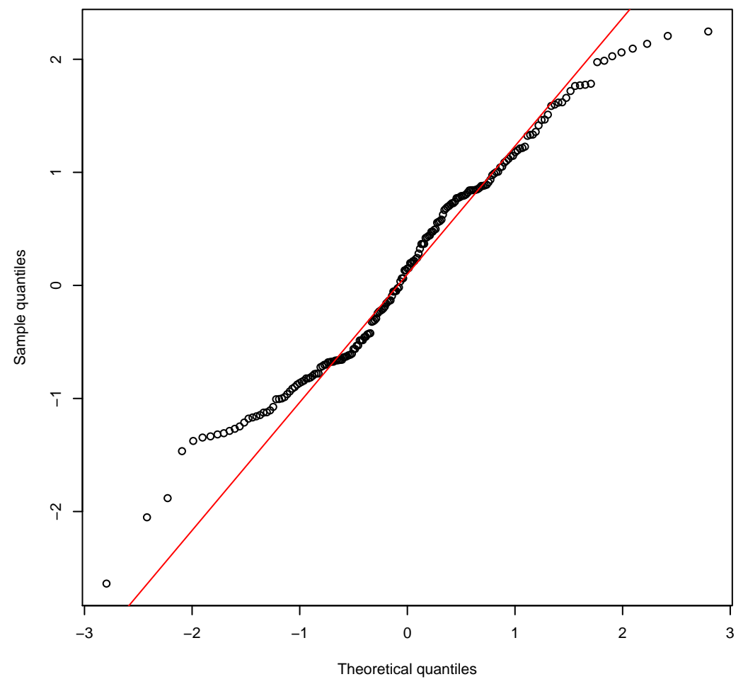
NB1 normal Q-Q plot
