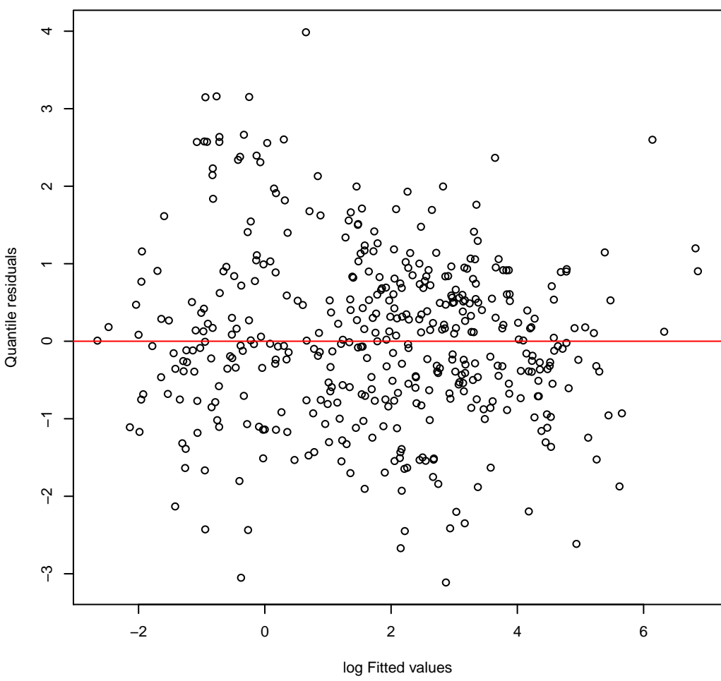
NB1 residual plot
