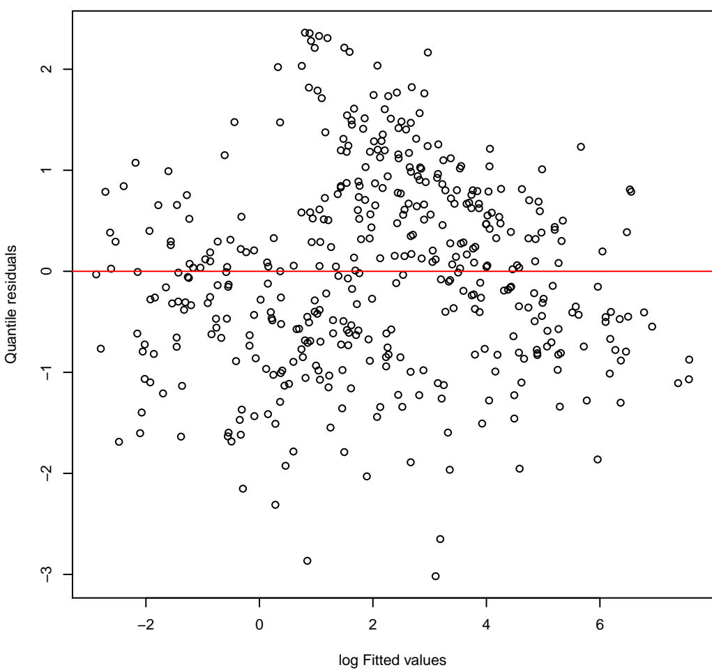
NB2 residual plot
