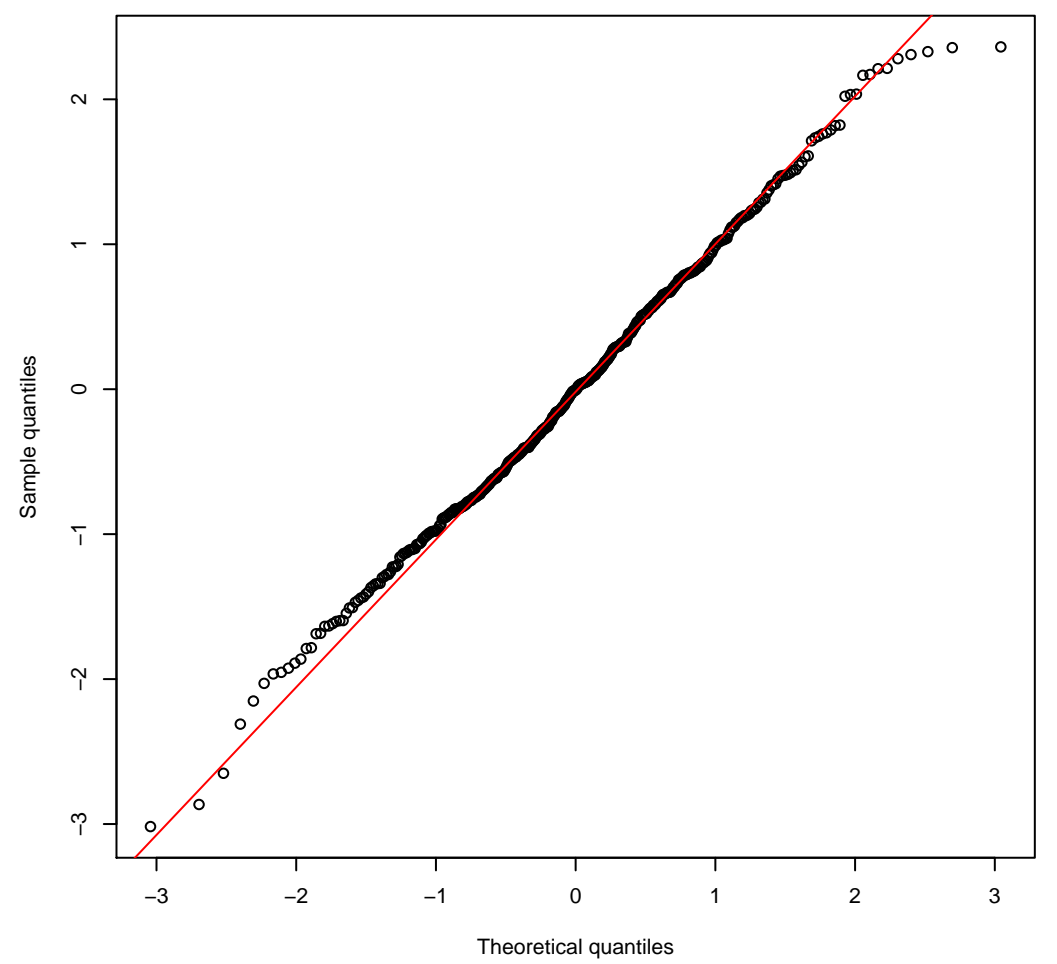
NB2 normal Q-Q plot
