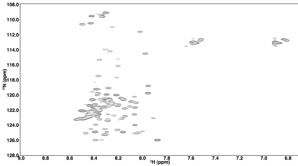
Figure S1. ^1\text{H} - ^{15}\text{N} HSQC spectrum of ProT \alpha in 400 g/L Ficoll 70. The sample contained 0.3 mM ProT \alpha in 50 mM NaPO _4 pH 7, 100 mM NaCl and 1 mM DTT.
