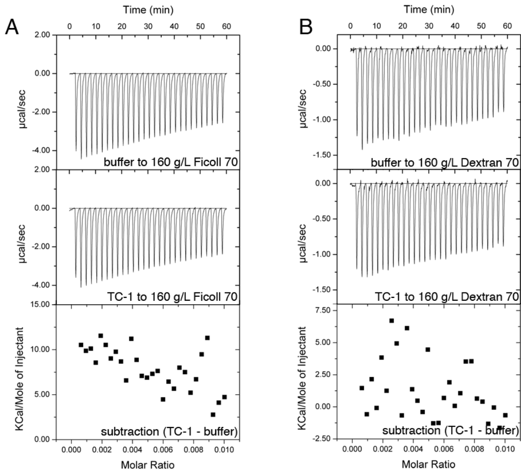
Figure S3. ITC profiles of TC-1 titrations into crowded solutions. Buffer (10 mM sodium acetate pH 5) alone or containing 0.1 mM TC-1 was titrated into the cell, containing 160 g/L Ficoll (A) or Dextran 70 (B) in the same buffer. 10 \mu\text{L} injections were used with 120-second delays.
