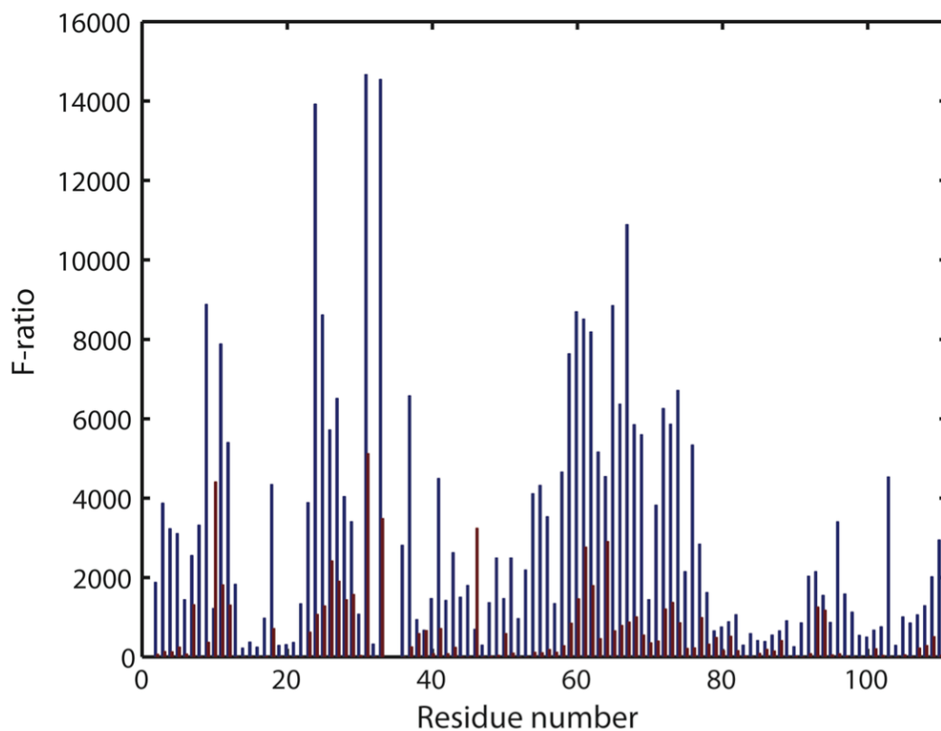
Figure S5. Comparison of the fitting of autocorrelations to 2-, 3-, and 4-exponential decay curves. Blue: F -ratios calculated from the \chi^2 and degrees of freedom of 2- and 3-exponential models; Red: F -ratios calculated from the \chi^2 and degrees of freedom of 3- and 4-exponential models (Equation 4).
