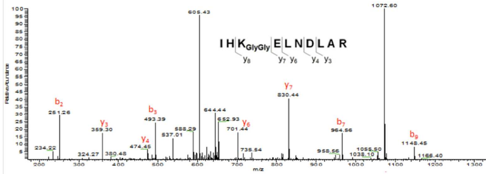
Supporting Figure 2 – Product ion spectrum for the doubly charged ubiquitinated peptide IHK GlyGly ELNDLAR.
