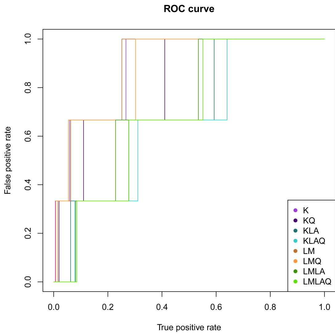
Figure S6 ROC curve of simulations with 3 causal SNPs, each adding phenotypic value 10, with a base phenotypic value given by one trait from (WARRINGER et al. 2011).
