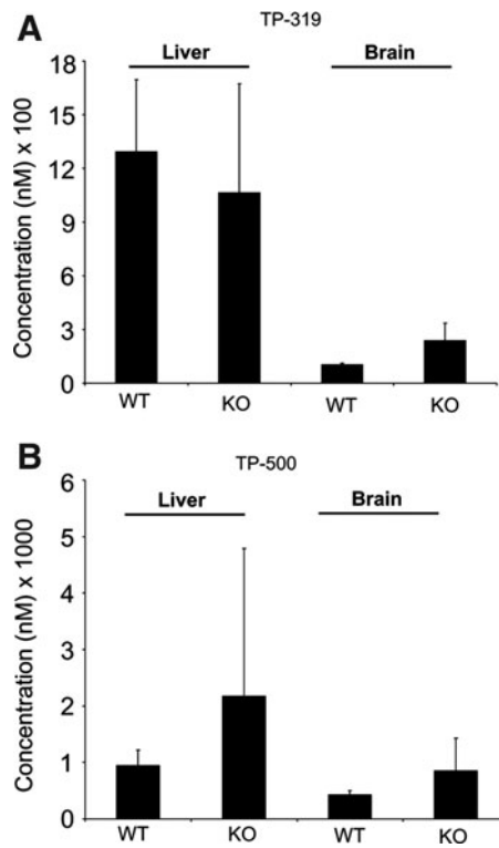
SUPPLEMENTARY FIG. S7. Relative levels of synthetic TP in vivo . (A) Levels of TP-319 and (B) levels of TP-500 in the liver and brain of WT and Nrf2 KO mice following two doses of 4 \mu mol of TP-319 administered 12 h apart by oral gavage and measured 9 h after the last dose. Bars represent mean \pm SDEV ( n=5 mice per group for each time point).
