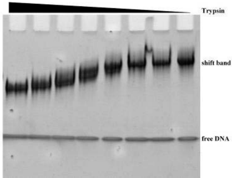
Figure S2 Gel shift assay analysis of the dTale2-DNA binary complex. After treatment with gradient concentrations (as indicated in experiment procedure) of trypsin on ice for 30 min, the dTale2-DNA binary complex was maintained.
