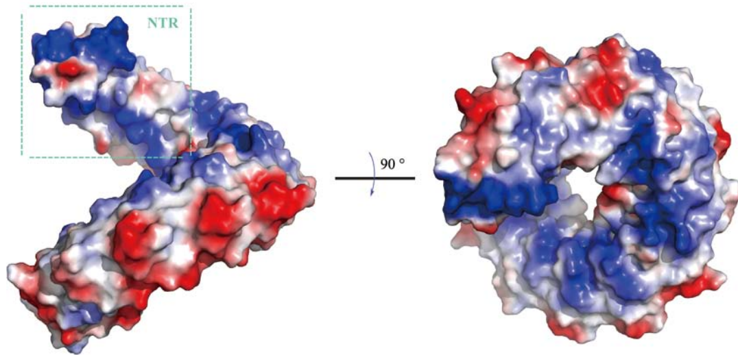
Figure S7 The electrostatic potential surface of dTale2. dTale2 (148-610), combined with the NTR and the CRD, is in surface representation and colored according to its electrostatic potential (positive potential, blue; negative potential, red).
