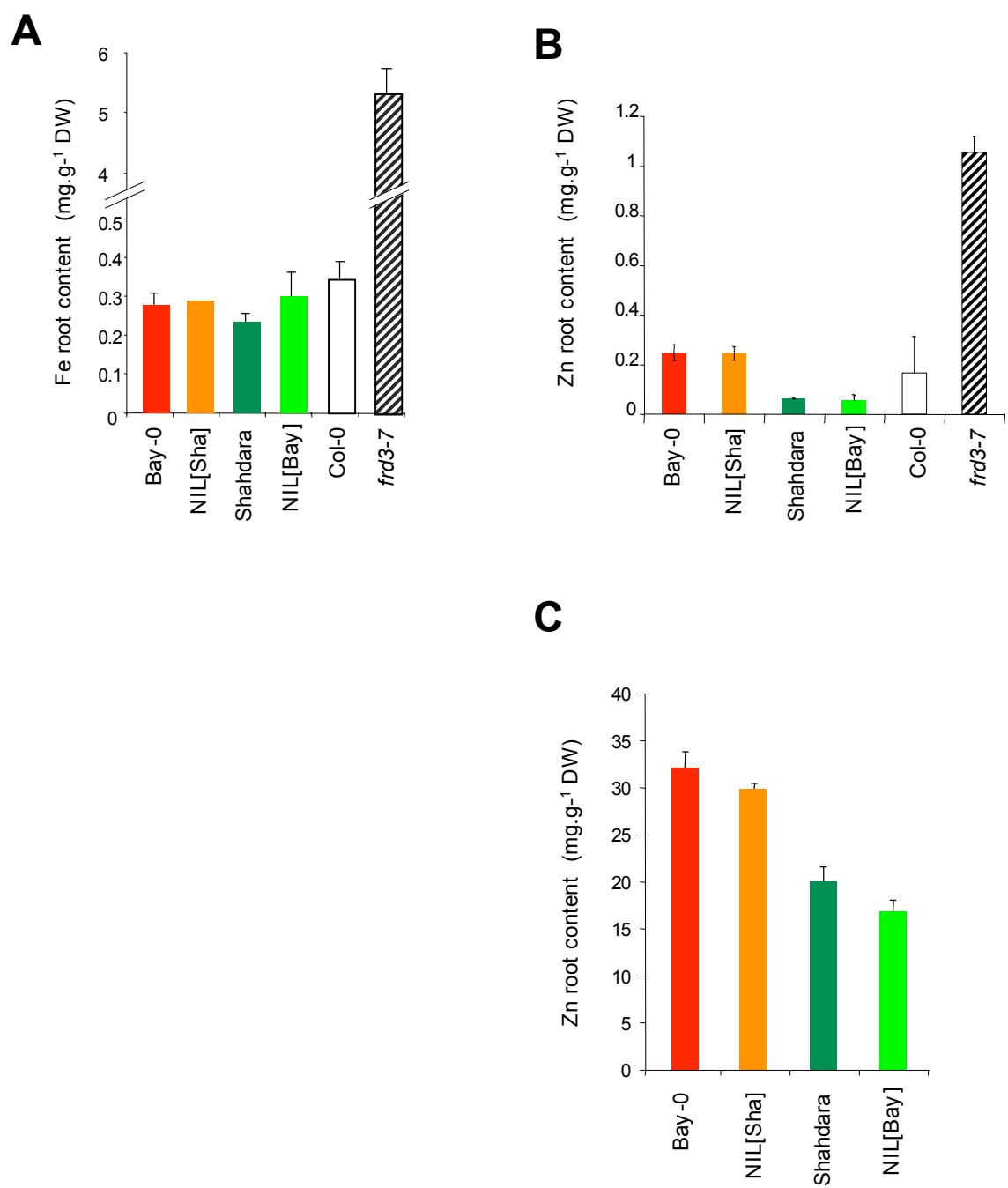
Figure S9
