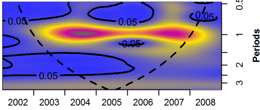
Wavelet power spectrum of district 316
