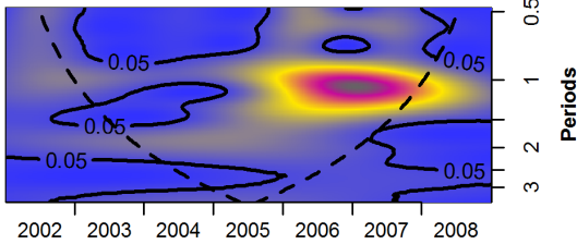
Wavelet power spectrum of district 402
