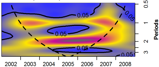
Wavelet power spectrum of district 203
