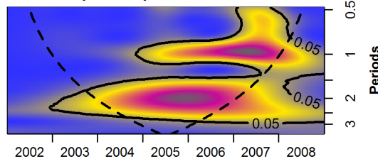
Wavelet power spectrum of district 212
