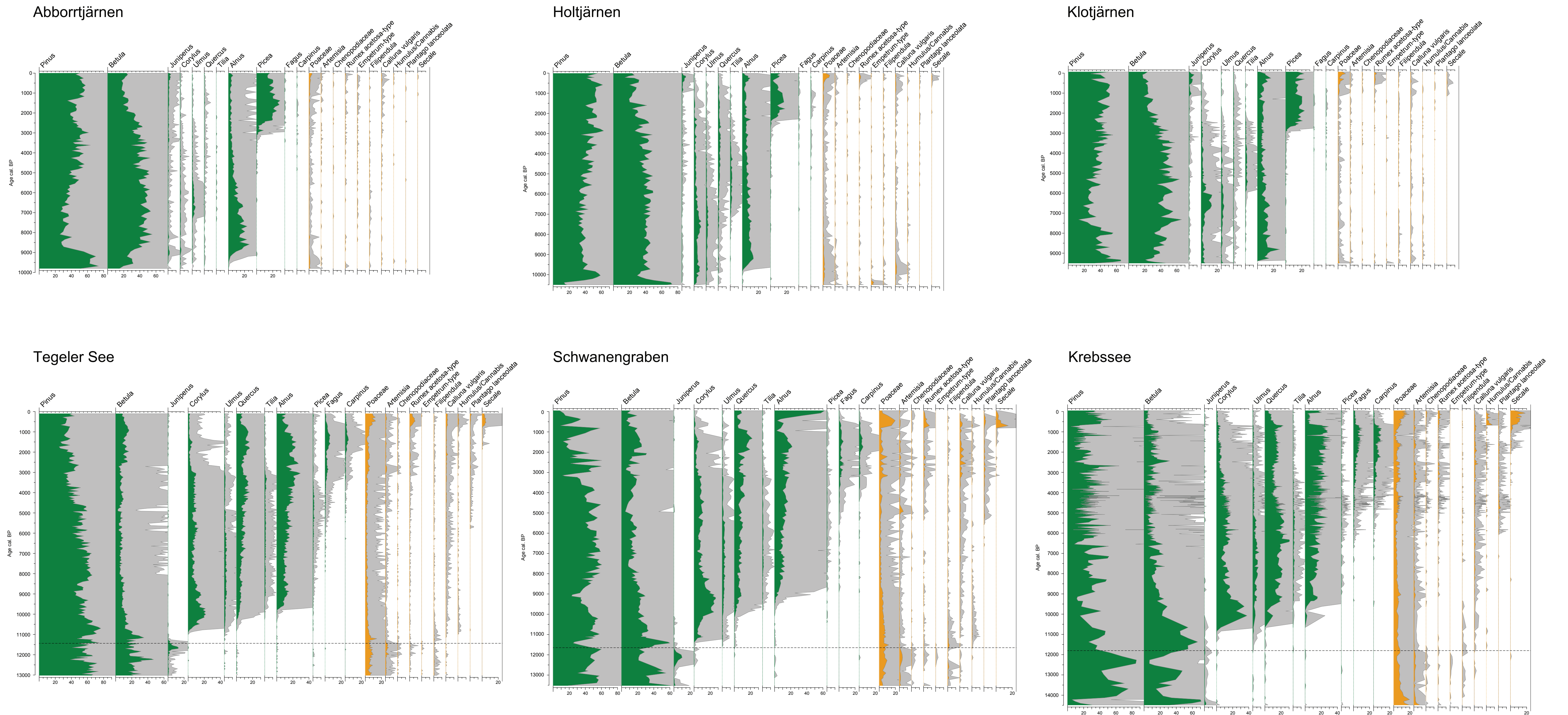
Figure S1. Percentage pollen diagrams showing a standardized set of selected taxa. The dotted lines in the diagrams from the southern sites mark the Holocene/Late-Glacial boundary as determined from pollen stratigraphy, which corresponds to slightly different ages at the three sites due to uncertainties in the age models.
