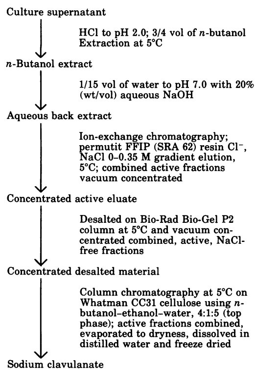
FIG. 3. Isolation of clavulanic acid as its sodium salt.
