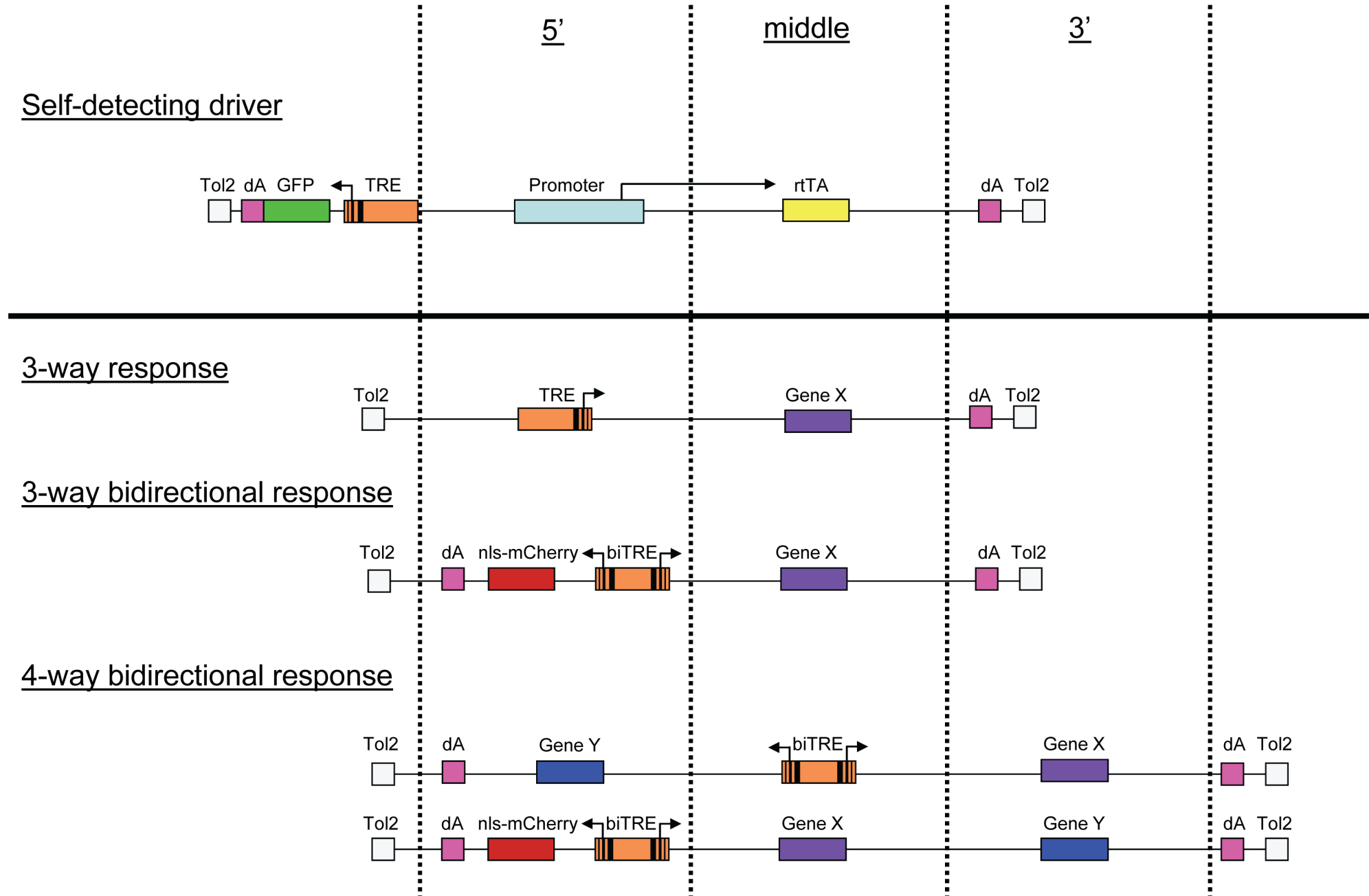
Figure S5. Possible Tet-On response vector conformations to use with self-detecting driver
