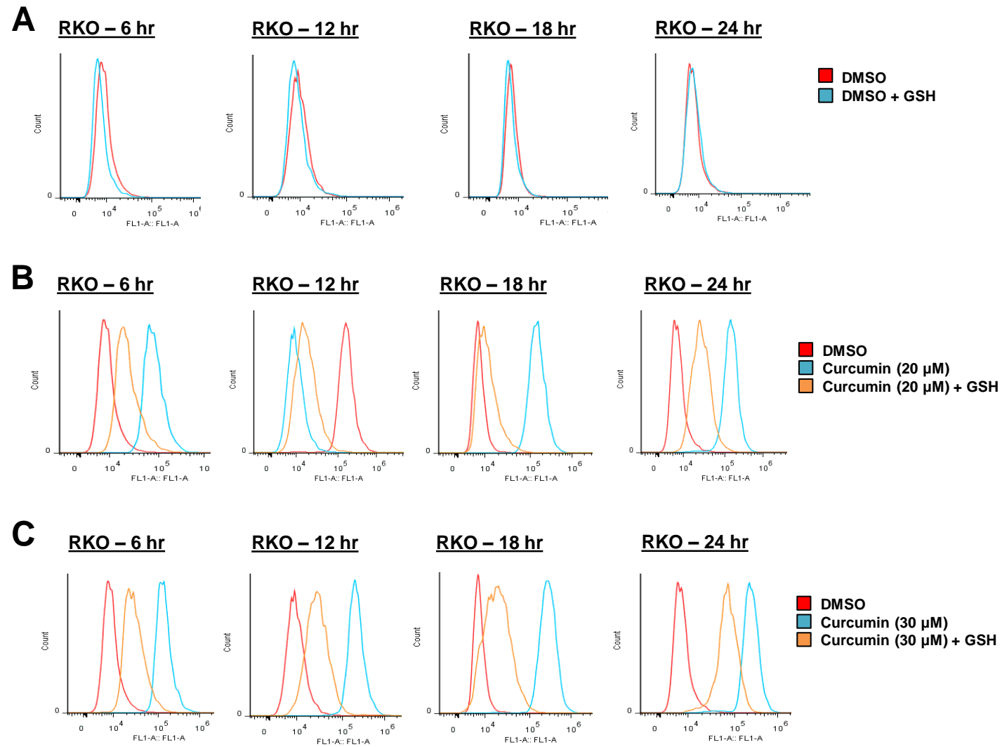
Supplemental Figure 2. ROS induction by curcumin. RKO cells were treated with 20 or 30 \mu M curcumin alone or with GSH. ROS was determined 6, 12, 18 or 24 hr after treatment by FACS analysis as outlined in the Materials and Methods.
