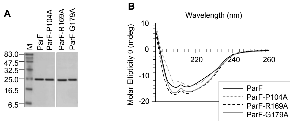
Fig. S1. (A) SDS-PAGE analysis of wild-type ParF and ParF-P104A, ParF-R169A and ParF-G179A proteins. Sizes of molecular weight markers (M) are indicated on the left (kDa). (B) Far UV circular dichroism spectra of wild-type ParF, ParF-P104A, ParF-R169A and ParF-G179A. The differences in the spectra between wild-type and mutated proteins are within the reproducibility limits of the technique.
