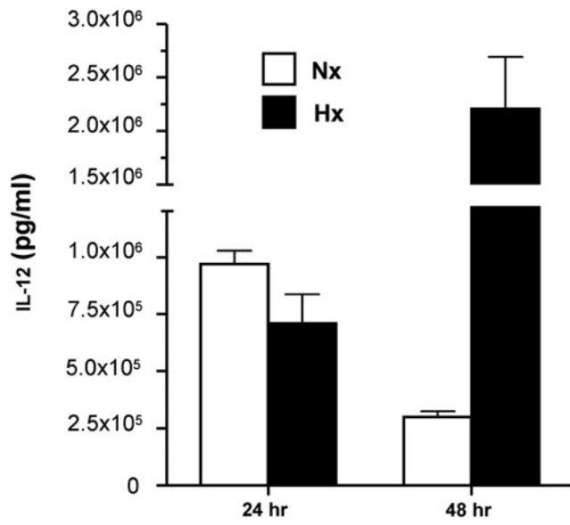
SUPPLEMENTARY FIG. S3. Expression of IL-12 in HM-1 cells infected with Ad-IL12G. HM-1 cells maintained under normoxic (Nx) or hypoxic (Hx) conditions were infected at a MOI 100 with Ad-IL12G. Production of IL-12 was quantified by ELISA in the supernatants 24 or 48 hr after infection.
