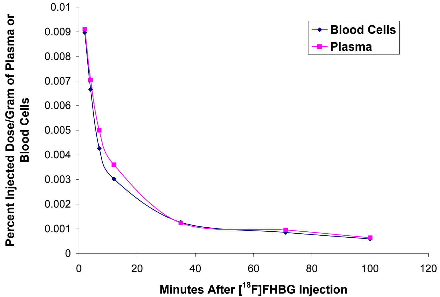
[ 18 F]FHBG Blood Time Activity Curve
