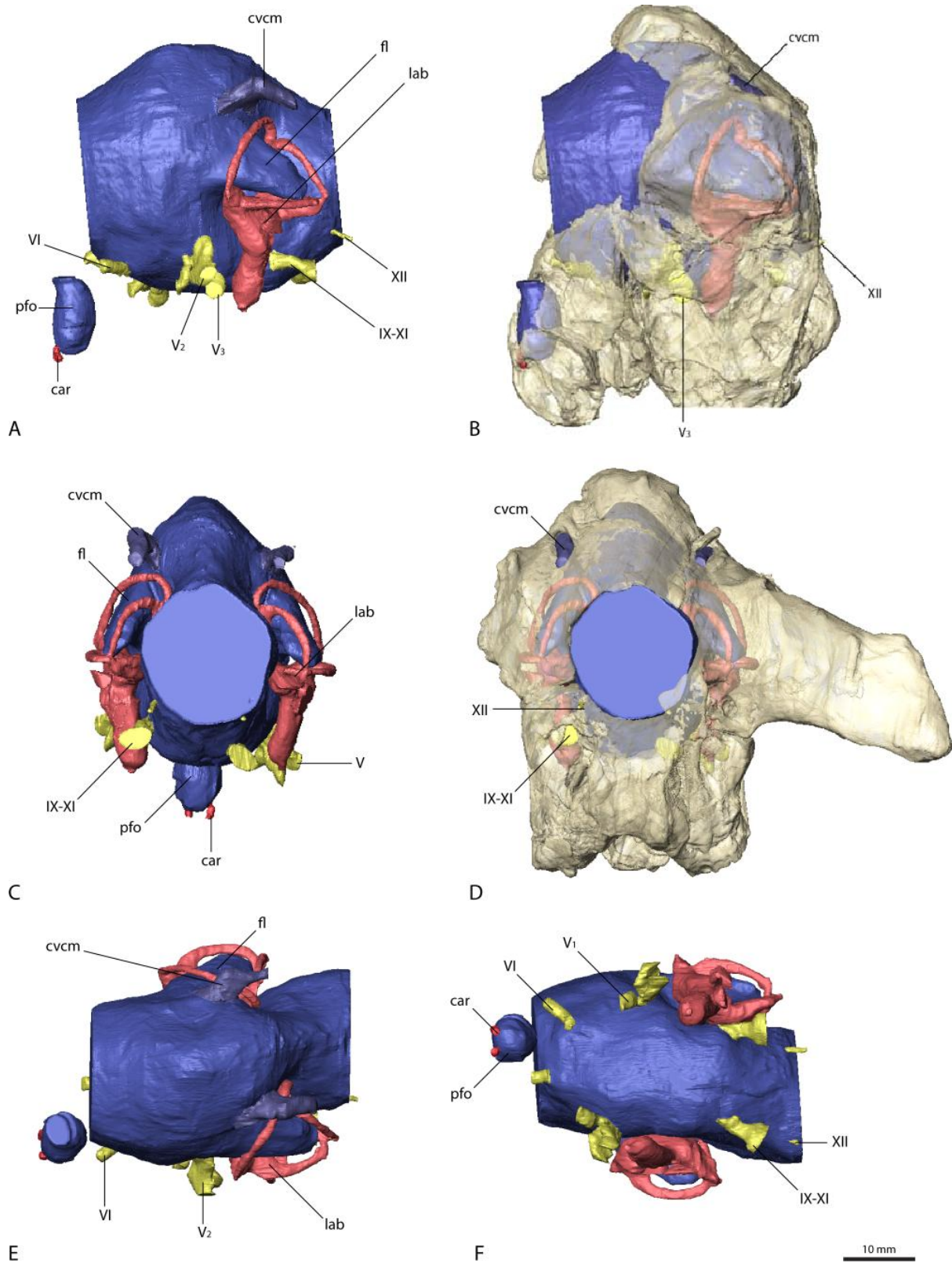
Figure S4. Cranial endocast and braincase of Falcarius utahensis (referred specimen, UMNH VP 15001). In (A) and (B) in left lateral, (C) and (D) in caudal, (E) dorsal, and (F) ventral view. Bone in (B) and (D) rendered transparent. Abbreviations: car, cerebral carotid artery canal; cvcm, caudal
