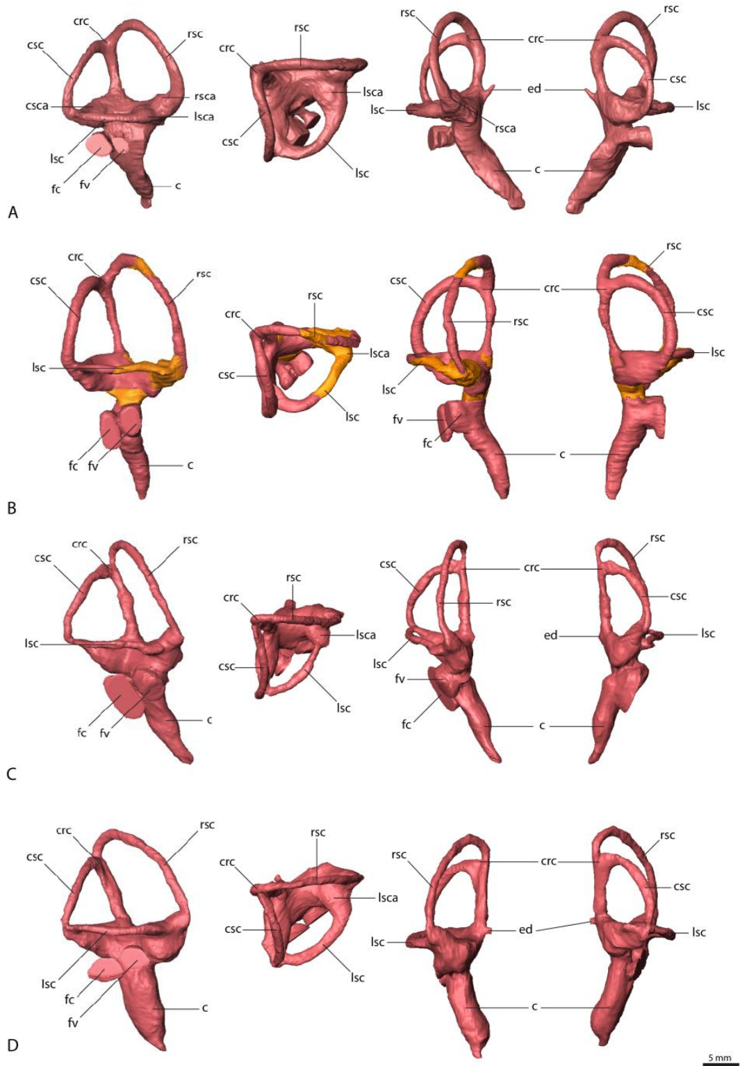
Figure S5. Endosseous labyrinths (right side). (A) Erlikosaurus andrewsi (IGM 100/111), (B) Nothronychus mckinleyi (AZMNH-2117, portions reconstructed from the left side shown in different color), (C) Falcarius utahensis (holotype specimen, UMNH VP 15000), (D) Falcarius utahensis (referred specimen, UMNH VP 15001). From left to right in lateral, dorsal, rostral and caudal view.
