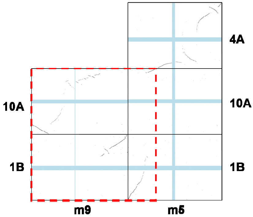
(G) See Fig. S4 and main text for details
