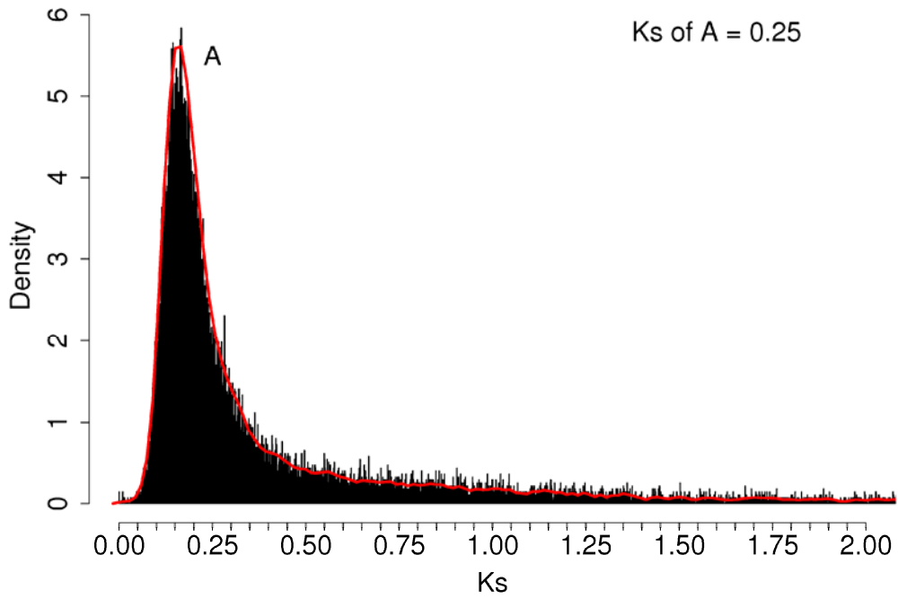
Figure S12: Ks values of gene pairs sharing mutual best BLASTP hits between sorghum and maize
