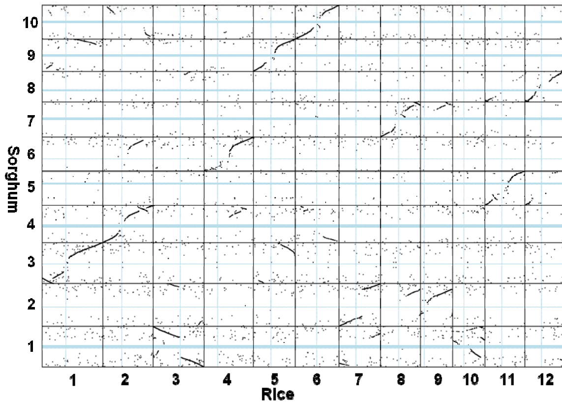
Figure S1: Sorghum-rice comparative map
