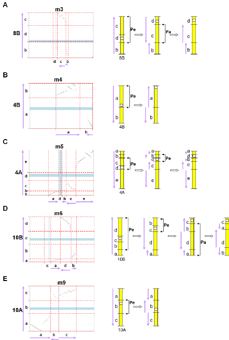
Figure S9: Models for centromere/pericentromere movement on Zea chromosomes during the descent of maize from a tetraploid ancestor.
