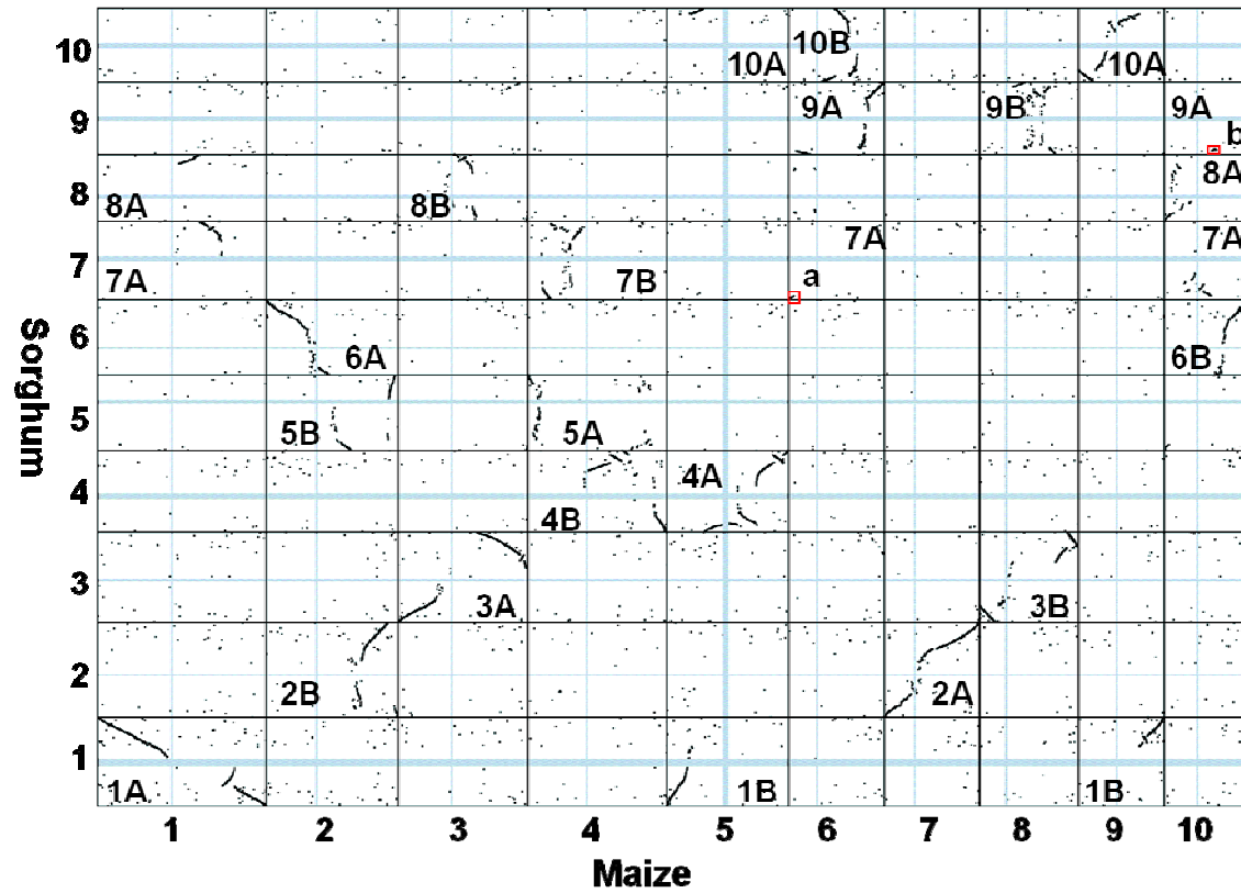
Figure S3: Sorghum-maize comparative map
