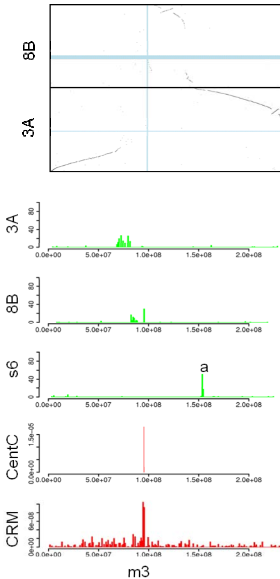
(C) Peak a related to centromere/pericentromere s6 corresponds to a region exhibiting a small synteny gap. This region may represent inter-chromosomal rearrangement of centromere/pericentromere s6 or assembly error. CSCP peaks related to centromere/pericentromere 8B cover maize cen3, which indicates that current maize cen3 originated from cen8B. Gene synteny patterns indicate movement of this centromere. The locations of CSCP peaks related to centromere/pericentromere 3A do not overlap with maize cen3A, indicating loss of this centromere (see main text for details).
