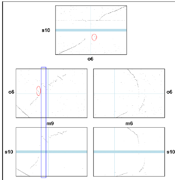
Figure S2: Differences between sorghum-maize and sorghum-rice comparative maps
