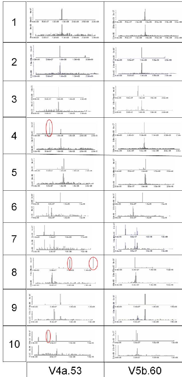
Figure S10: CentC/CRM distribution in two maize assemblies
