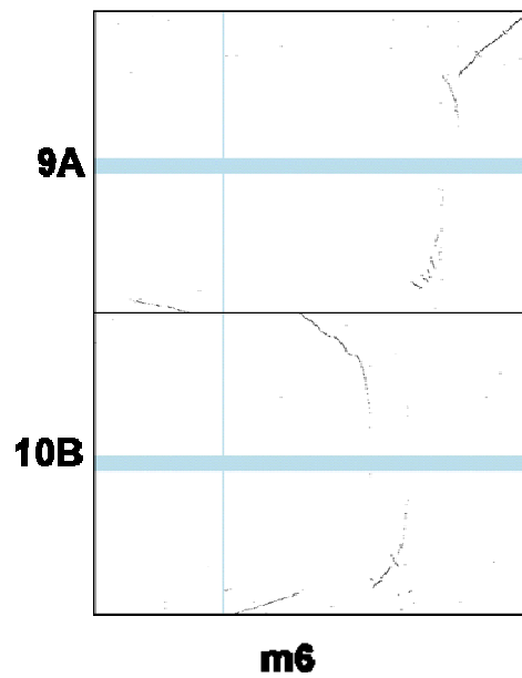
(D) Not considering the 5' end (region a in Fig. S3), m6 originated by insertion of 10B into 9A.
