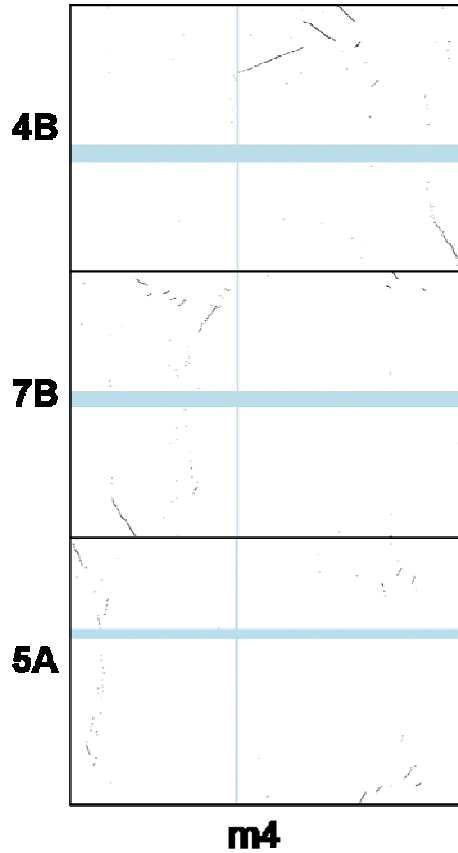
(C) M4 originated by two fusions: 5A with 7B and 7B with 4B. Extensive intra-chosomal movements can be seen.
