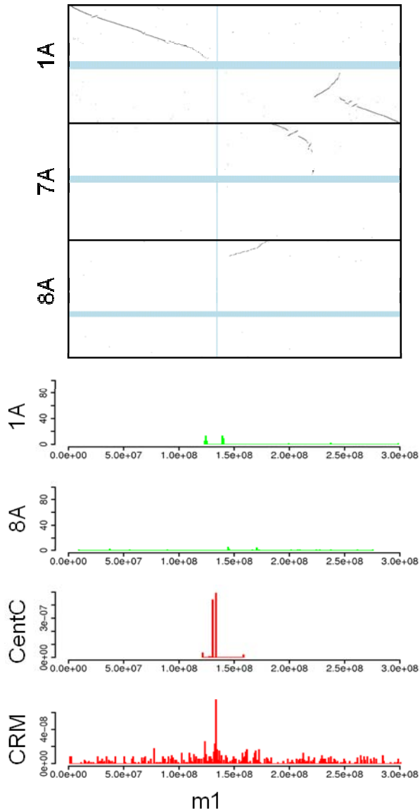
Figure S8: Relationships of current and ancient centromeres/pericentromeres between sorghum and maize
