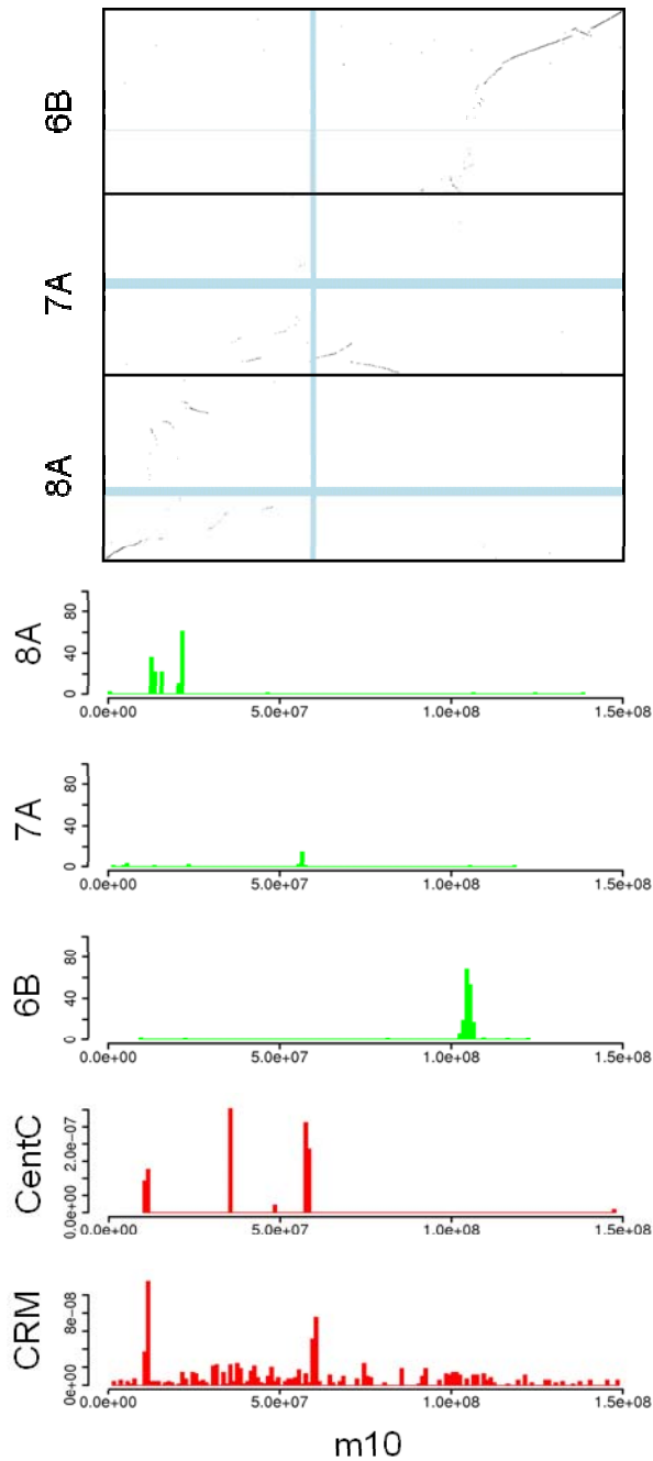
(J) A CentC peak is found at 34Mb - 36Mb. It may be artificial peak caused by assembly error (Fig. S10). The peak located at 11Mb - 13Mb corresponds to ancient centromere/pericentromere 8A. This peak is relocated in assembly release 5b.60 (Fig. S10). Current maize cen10 overlaps with centromere/pericentromere 7A, so it is likely to have originated from cen7A.
