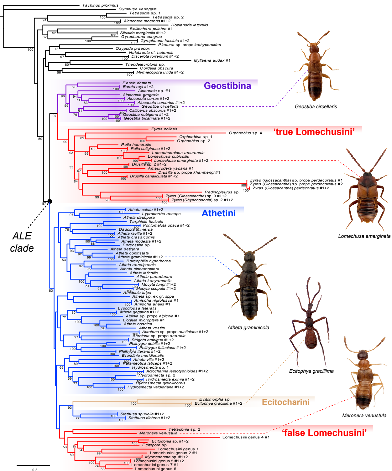
Supplementary Figure S1 Best tree from the Maximum Likelihood analysis with incomplete sequences excluded. Bootstrap values \geq 50\% are indicated under the branches. The labels of conspecific specimens have been combined to save space.
