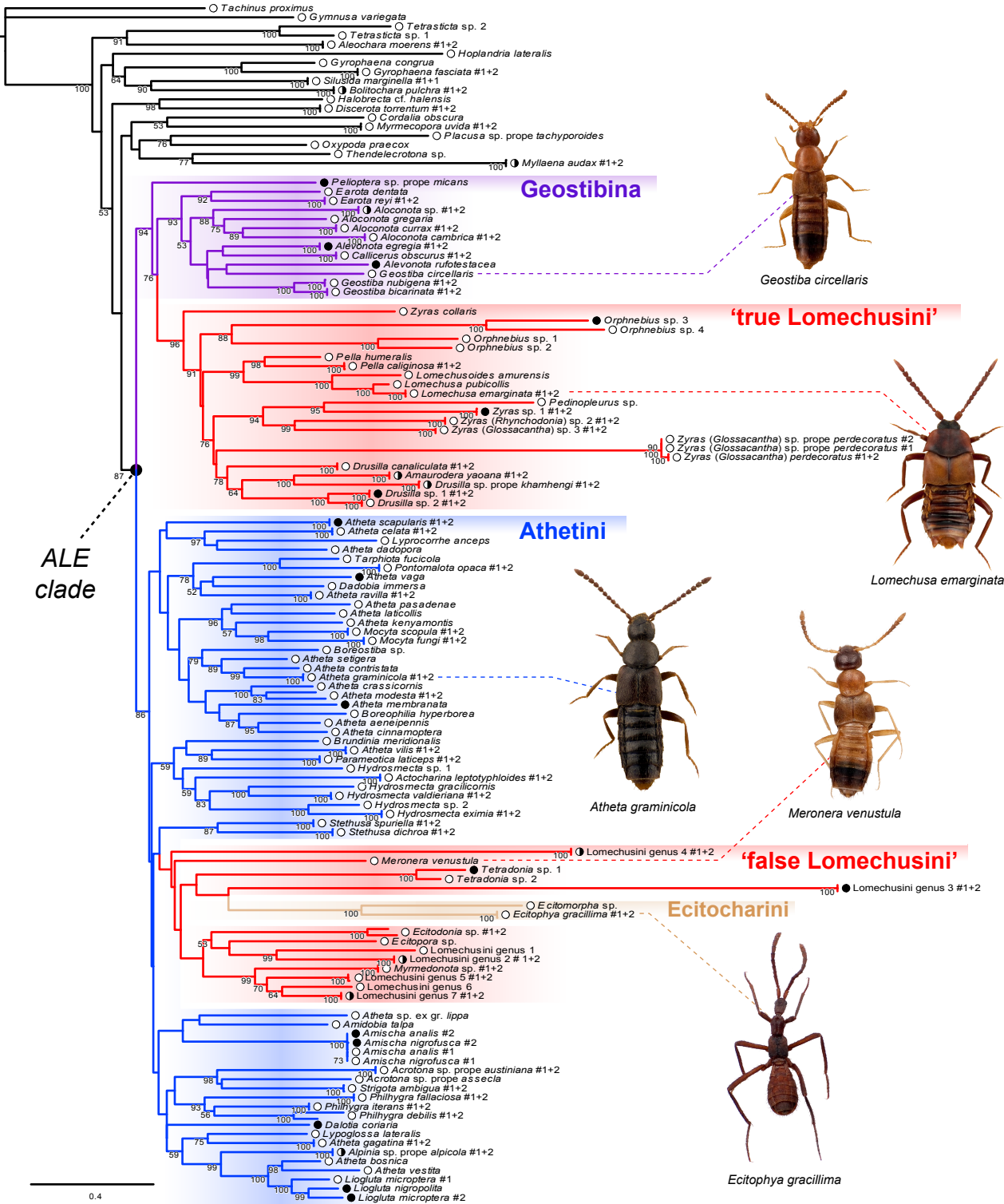
Supplementary Figure S2 Best tree from the Maximum Likelihood analysis with incomplete sequences included. Bootstrap values \geq 50\% are indicated under the branches. The labels of conspecific specimens have been combined to save space, except where the specimens did not group together. Complete sequences are indicated with open circles, incomplete with solid circles. Half-solid circles indicate pairs of conspecific specimens with one having incomplete sequence.
