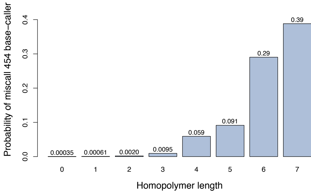
Figure 1: Probability of miscalls by the native 454 base-caller for different HPLs. The base-calling error rate clearly increases by increasing HPL and becomes quite substantial from HPL 4.
