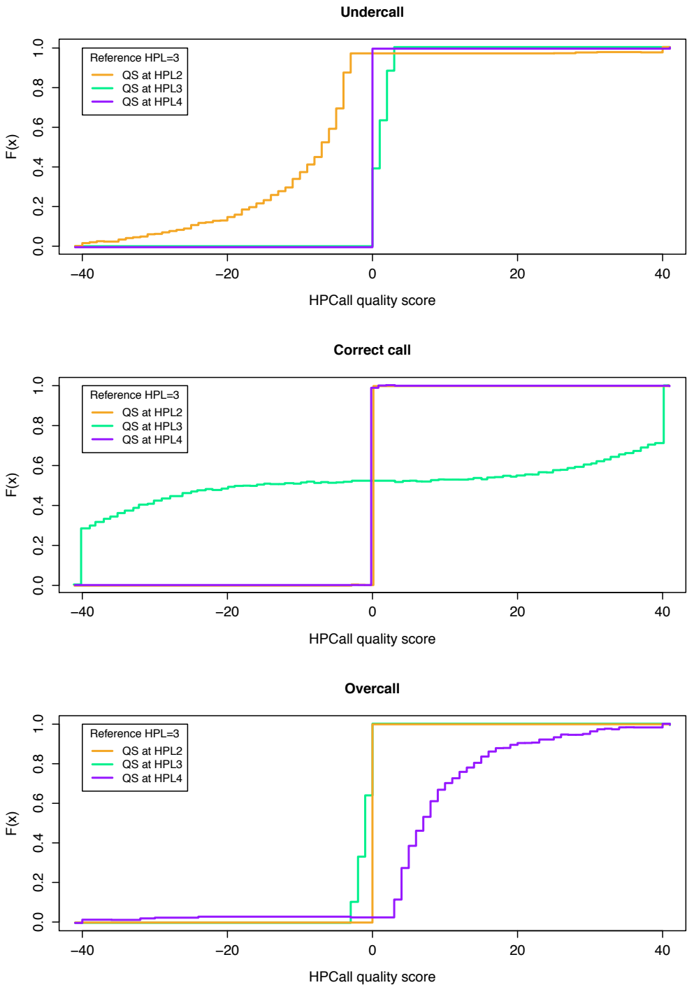
Figure 4: The empirical cumulative distribution function of HPCall quality scores QS_{\text{HPCall}} for sequences with reference HPLref 3 assigned to bases associated with HPL 2, 3 and 4, in the case of an undercall (upper), correct call (middle) or overcall (lower).
