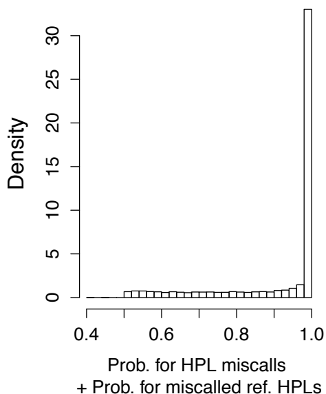
Figure 5: (A) Histograms of the maximal estimated probabilities by HPCall in the case of a correct call (upper left), and (B) in the case of a miscall (upper right). (C) The histogram in the lower left panel gives the distribution of estimated probabilities for the reference HPLs in the case of a miscall. These very often correspond with the reference HPL. (D) The lower right panel gives the histogram of the sum of the probabilities given in the upper right and lower left panel. These two probabilities almost always sum to a value close to 1.
